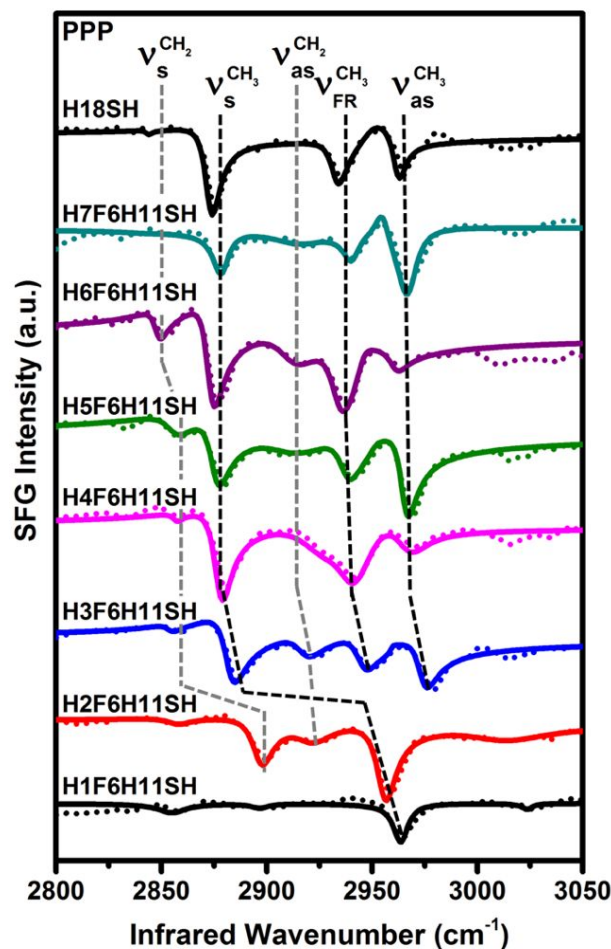
Figure 6. Normalized SFG spectra for the C-H stretching region collected from H n F6H11SH FSAMs. The solid lines denote the fits to the spectra according to Equation S1. PPP denotes the polarization direction of the SFG, visible, and IR beams, in that order, with respect to the surface normal. The symmetric, \nu_s^{\text{CH}_3} , and antisymmetric, \nu_{\text{as}}^{\text{CH}_3} , methyl C-H stretching peak positions are marked with black dotted lines. The SFG spectrum of H18SH is included as a reference.
