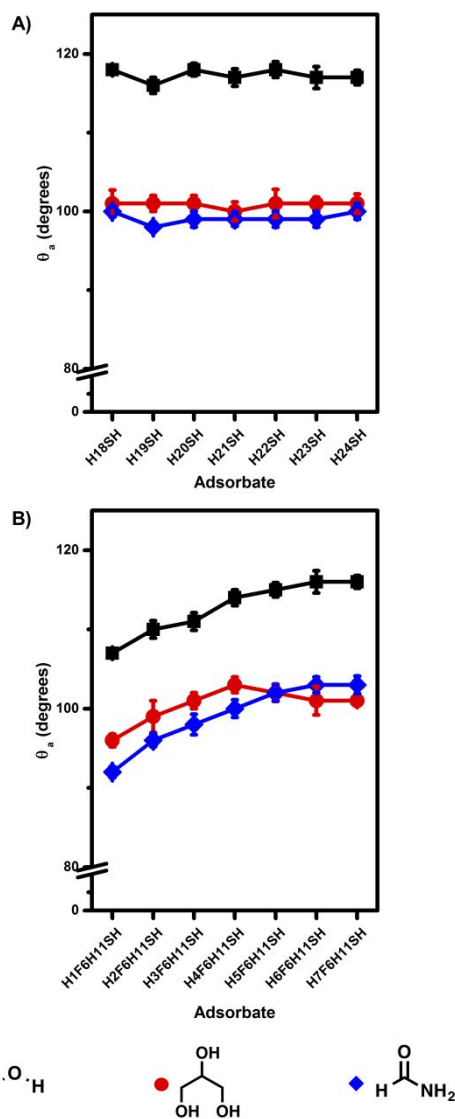
Figure 11. Advancing contact angle values of the polar protic liquids on (A) the HmSH SAMs and (B) the HnF6HnSH FSAMs. Small error bars lie within the symbol.
