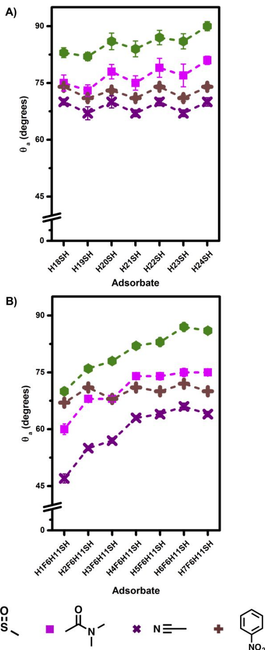
Figure 10. Advancing contact angle values of the polar aprotic liquids on (A) the HmSH SAMs and (B) the HnF6HnSH FSAMs. Small error bars lie within the symbol.
