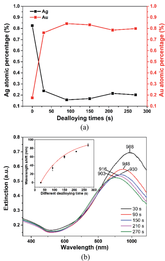
Fig. 2 Elemental composition and extinction spectra of 300 nm diameter NPG disk made from \text{Ag}_{82.5}\text{Au}_{17.5} alloy: (a) atomic percentage of Ag and Au versus dealloying time. (b) extinction spectra versus dealloying time. The inset shows blueshift versus dealloying time. The curve is only for visual guidance.
