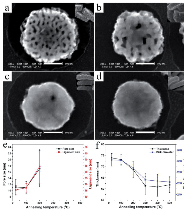
Fig. 4 SEM images of NPG nanoparticles after different annealing temperature: (a) 100, (b) 200, (c) 300, and (d) 400 °C. The insets show thickness. (e) the changes of pore and ligament size versus annealing temperature, and (f) is the thickness and NPG disk diameter versus annealing temperature. SEM scale bar: 100 nm.
