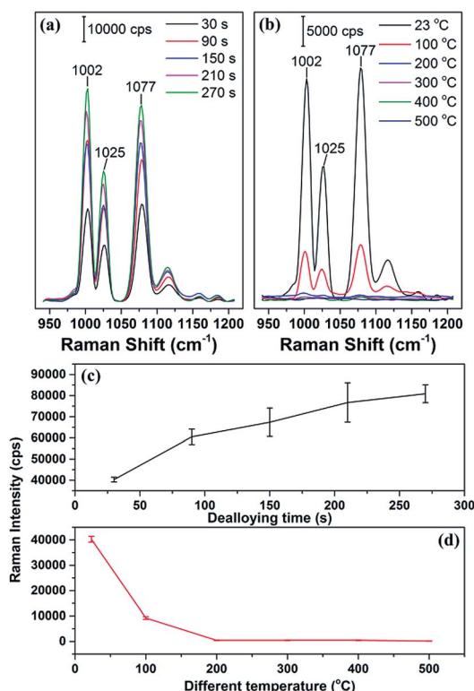
Fig. 7 Surface-enhanced Raman spectra of benzenethiol ranging from 930 to 1210 \text{ cm}^{-1} on NPG nanoparticles obtained from \text{Ag}_{82.5}\text{Au}_{17.5} alloy: (a) different dealloying time and (b) different annealing temperatures for NPG nanoparticles obtained after 30 s dealloying; (c) and (d) are the change trends of intensity of the SERS band at 1077 \text{ cm}^{-1} corresponding to different dealloying time and temperatures, respectively.
