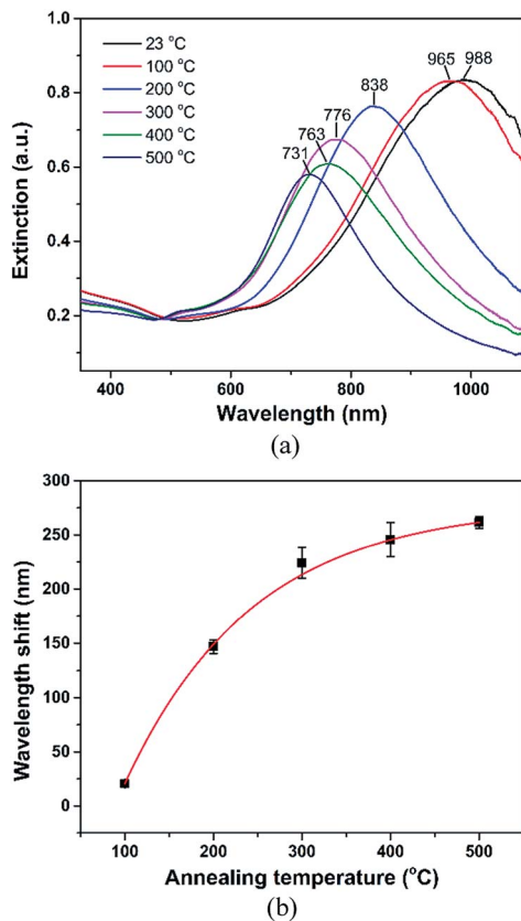
Fig. 5 Extinction spectra of 300 nm as-dealloyed NPG nanoparticles from \text{Ag}_{82.5}\text{Au}_{17.5} alloy at 30 s before and after annealing: (a) extinction bands after annealing at different temperatures and (b) the wavelength blueshift as a function of annealing temperatures.
