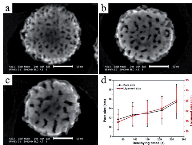
Fig. 1 SEM images and image analysis of 300 nm diameter NPG nanoparticles made from \text{Ag}_{82.5}\text{Au}_{17.5} alloy for different dealloying time: (a) 30, (b) 150 and (c) 270 s. (d) pore and ligament sizes based on statistical analysis versus dealloying time. SEM scale bar: 100 nm.
