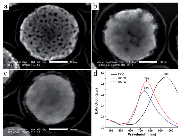
Fig. 6 SEM images of ~300 nm NPG nanoparticles dealloyed at 90 s from \text{Ag}_{70}\text{Au}_{30} alloy at (a) 23 °C, (b) 200 °C and (c) 300 °C. (d) Extinction spectra at corresponding temperatures. SEM scale bar: 100 nm.
