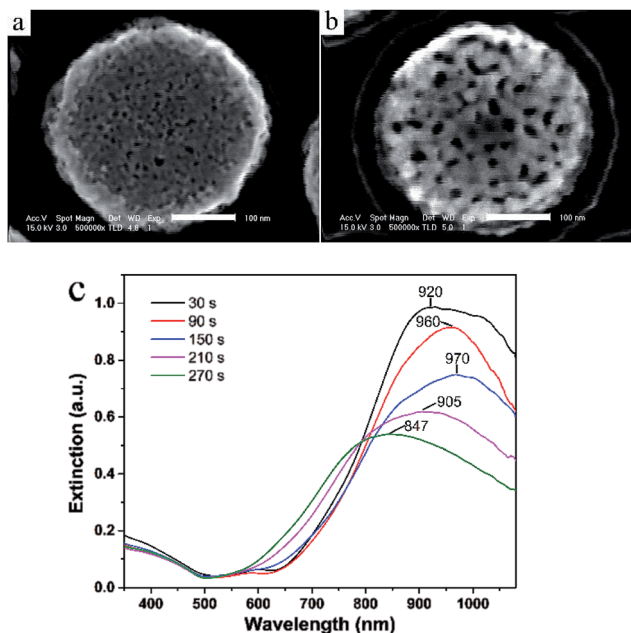
Fig. 3 SEM images and extinction spectra of \sim 300 nm diameter NPG disk made from \text{Ag}_{70}\text{Au}_{30} alloy: (a) and (b) are the SEM images of NPG disk at 30 s and 270 s, and (c) extinction spectra versus dealloying time. SEM scale bar: 100 nm.
